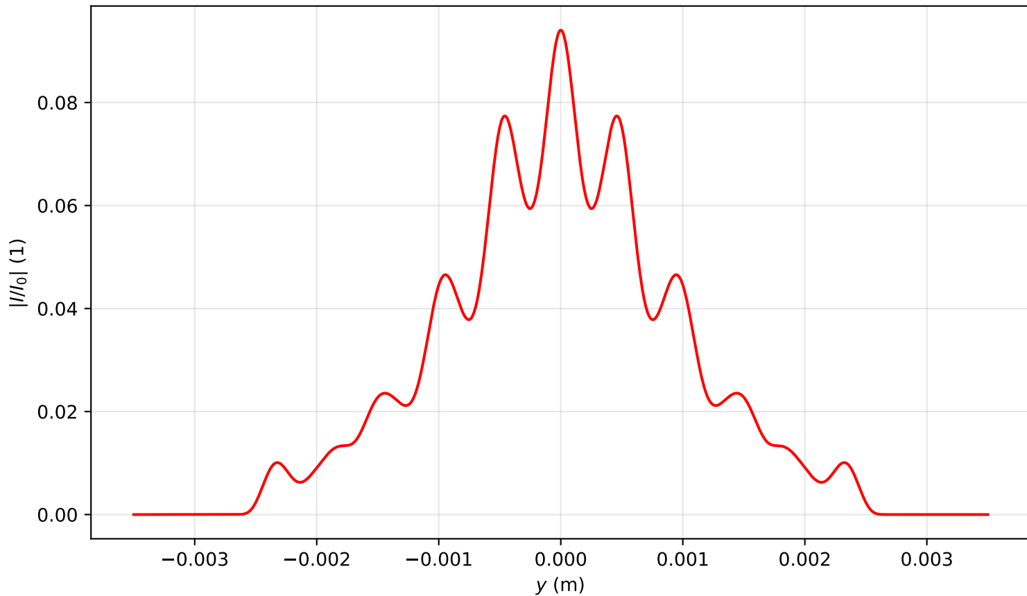
Intensity profile I(x=0, y, z=3.503)/I_0 , P_{in}=2.0P_{cr} , artificial time
